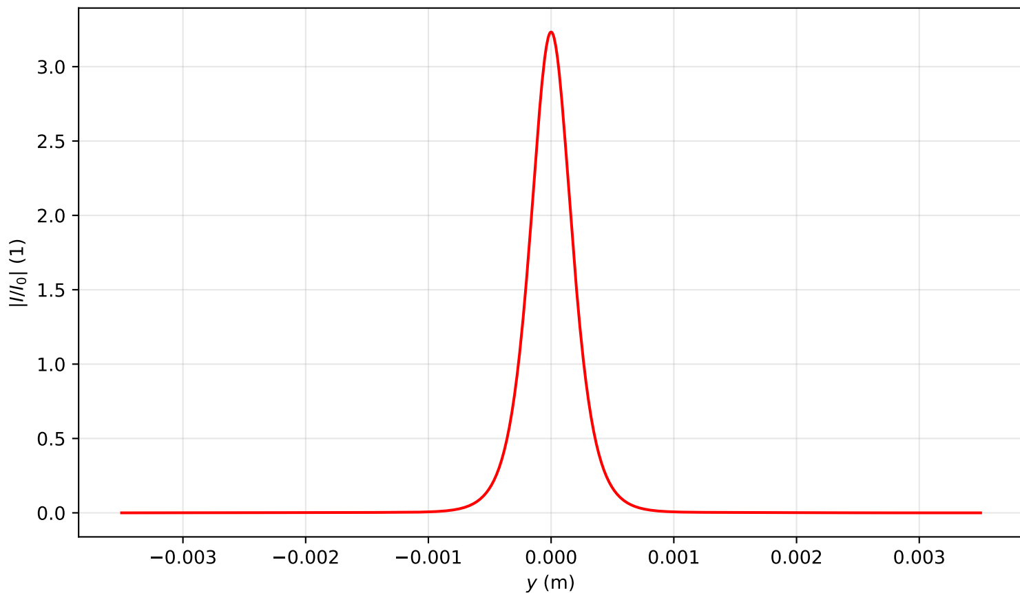
Intensity profile I(x=0, y, z=3.821)/I_0 , \text{Pin}=1.0\text{Pcr} , artificial time
